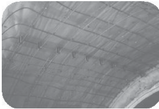
Preshaped Girders
